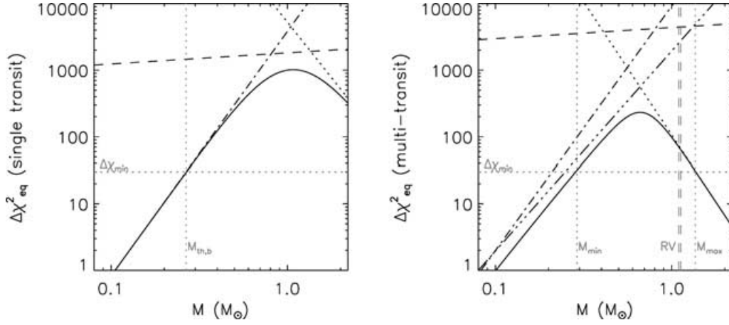
Figure 2. Detection statistic \Delta\chi^2_{\text{eq}} for an equatorial transit, for individual transits and assuming the systematics are white (as in PG05a, left-hand panel) or for multiple transits and incorporating both red noise terms with \sigma_{\text{sys}} = 1.5 mmag and k = 0.2 (this work, right-hand panel). The line styles have the same meaning as in Fig. 1. The grey horizontal dotted line marks the detection threshold \Delta\chi^2_{\text{min}} = 30 adopted by PG05a. The grey vertical dotted lines mark the lower and, if applicable, upper mass limits between which the transits are detectable. The grey vertical dashed lines mark the mass range where RV follow-up is feasible with FLAMES + UVES.
