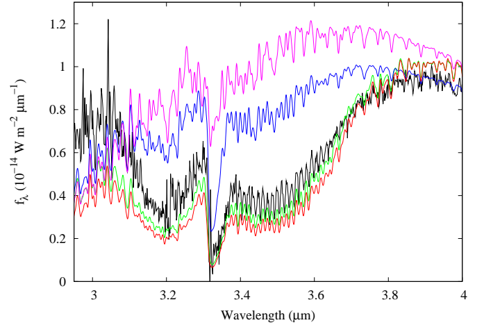
Fig. 26. The L -band spectrum of \epsilon Indi Ba (black line) and different chemistry models with T_{\text{eff}}=1320 K, \log g=5.50 , [M/H]=-0.2 . A chemical equilibrium model is shown in green, the Prinn & Barshay (1977) model in blue, the Prinn & Barshay (1977) model with the revised reaction rates of Griffith & Yelle (1999) in magenta, and a model following the Yung et al. (1988) chemistry in red. All models have been smoothed to 60 Å FWHM to match observations.
