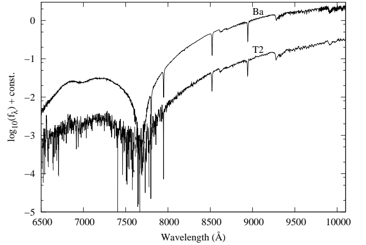
Fig. 10. Optical spectrum of \varepsilon Indi Ba and the T2 (SDSS 1254-0122 (Burgasser et al. 2003)) optical spectral standard. There is no object defined as either the T0 or T1 spectral standard in the optical. The \varepsilon Indi Ba spectrum is normalised to unity at 9000 \text{ \AA} and the T2 standard spectrum is offset by 1 dex for clarity.
