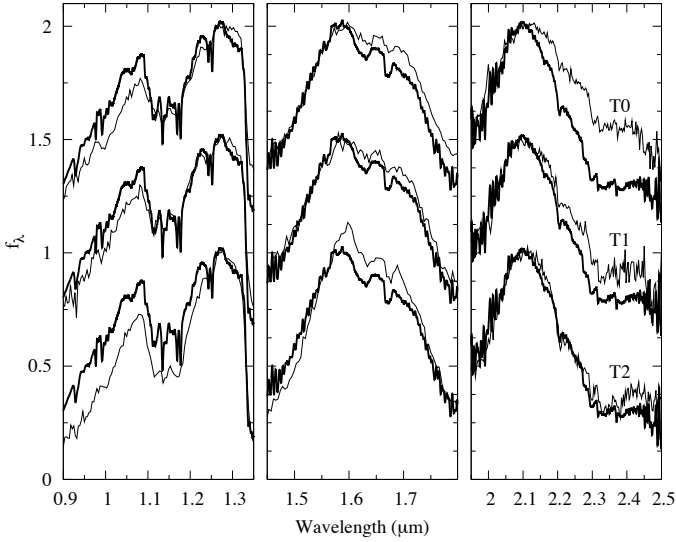
Fig. 8. Smoothed spectrum (30 Å FWHM) of \epsilon Indi Ba (thick lines) and spectra of the T0 (SDSS 120747.17+024424.8; Looper et al. 2007), T1 (alternate standard SDSS 015141.69+124429.6; Burgasser et al. 2004), and T2 (SDSS J125453.90-012247.4; Burgasser et al. 2004) spectral standards. The three panels show the JHK bands omitting the lower signal-to-noise H 2 O absorption regions between the bands. Spectra are normalised to unity at 1.27 \mu m in the J -band, at 1.58 \mu m in the H -band, and at 2.10 \mu m in the K -band and offset to show the \epsilon Indi Ba spectrum against each of the spectral standards.
