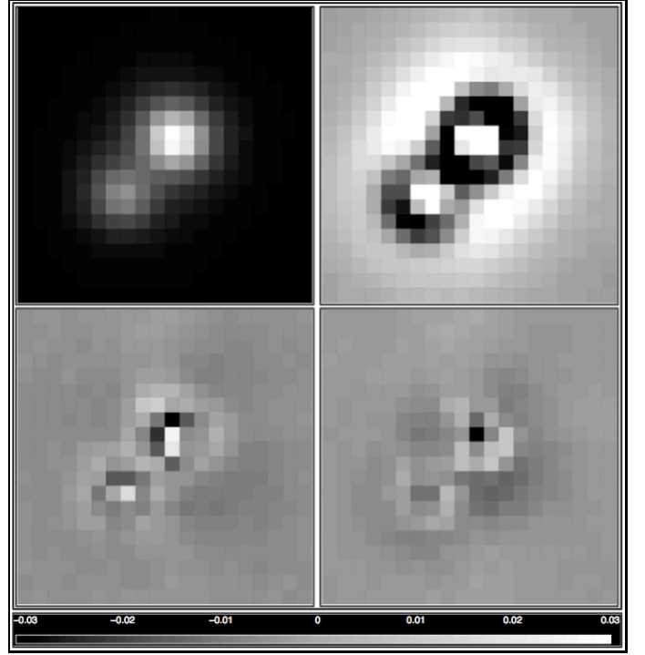
Fig. A.1. An ISAAC J -band image of the \epsilon Indi Ba, Bb system (top left) and the residuals of the Gaussian (top right), modified Lorentzian (bottom left), and Moffat profile fits (bottom right). Each image is a 20 \times 20 pixel ( 2.96'' \times 2.96'' ) sub-section of the full image. North is up, East left. The scale applies to the residual images and shows the flux as a fraction of the observed peak pixel flux. It is apparent that the Gaussian profile is the worst fit, while the Moffat profile is somewhat better than the Lorentzian.
