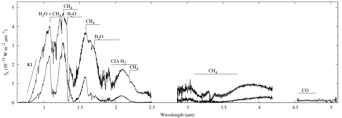
Fig. 3. Full 0.6–5.1 \mu\text{m} spectrum of \varepsilon Indi Ba and Bb (upper and lower lines respectively). Here the full resolution optical and near-IR spectra have been smoothed to 17 \text{\AA} FWHM to allow inspection of the broad features without being dominated by the many fine features seen in the full resolution spectra (see Figs. 5–7).
