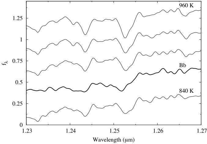
Fig. 19. 1.23\text{--}1.27 \mu\text{m} spectrum of \epsilon Indi Bb (thicker line, second from bottom) and the [M/H]=-0.2 , \log g=5.25 BT-Settl spectra with T_{\text{eff}}=840\text{--}960 K (increasing bottom to top in steps of 40 K). All spectra have been normalised and offset for clarity. All spectra have been smoothed to 10 \text{ \AA} FWHM for easier comparison.
