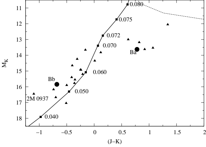
Fig. 12. M_K -( J-K ) colour-magnitude diagram with the 5 Gyr COND03 isochrone (Baraffe et al. 2003) with masses (in M_\odot ) indicated as filled squares. The DUSTY00 5 Gyr isochrone (Chabrier et al. 2000) is also shown (upper, dashed line). The positions of \epsilon Indi Ba and Bb are marked with filled circles, the filled triangles show the T dwarf observations of Knapp et al. (2004) and Chiu et al. (2006), and the metal-poor T6 subdwarf 2MASS 0937+2931 is labelled. All magnitudes are in the MKO system. We do not show isochrones for different ages as they show little variation in position, except that the same masses correspond to different magnitudes.
