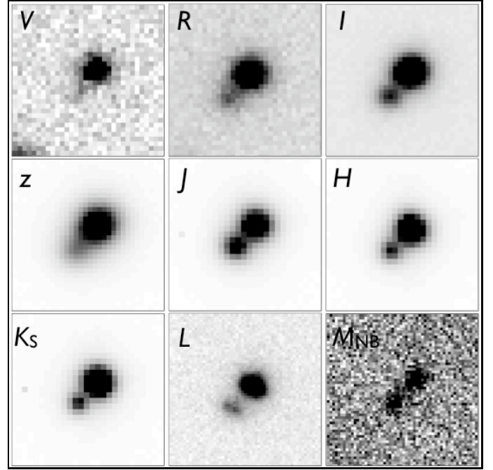
Fig. 1. From left to right and top to bottom, FORS2 VRIz and ISAAC JHK_SLM_{NB} images of \epsilon Indi Ba, Bb. Each image is a 4'' \times 4'' subsection of the full image. North is up, East left. The object to the south-east of the V -band image is a faint galaxy not seen in the other passbands. The L -band profiles are seen to be slightly elliptical. The V and M_{NB} -band images are the stacked images of all observations in those passbands.
