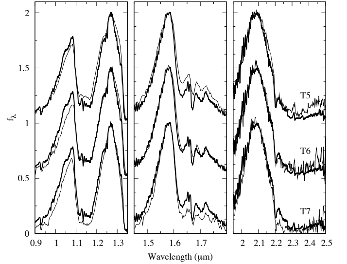
Fig. 9. Smoothed spectrum (30 Å FWHM) of \epsilon Indi Bb (thick lines) and spectra of the T5 (2MASS 15031961+2525196; Burgasser et al. 2004), T6 (SDSS 162414.37+002915.6; Burgasser et al. 2006a), and T7 (2MASS 0727182+171001; Burgasser et al. 2006a) spectral standards. Plotted regions and normalisation are as in Fig. 8.
