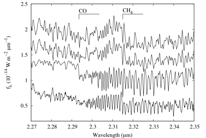
Fig. 25. The 2.27–2.35 \mu\text{m} spectrum of \epsilon Indi Ba (bottom line) showing the CO 2–0 overtone along with models employing different chemical equilibrium (CE) timescales. All models have T_{\text{eff}}=1320 K, \log g=5.50 , and [M/H]=-0.2 . A chemical equilibrium model is shown at the top, the Prinn & Barshay (1977) model second from bottom, and a model following the Yung et al. (1988) chemistry second from top. All models have been smoothed to 4.9 Å FWHM to match the observations. The \epsilon Indi Ba spectrum shows the absolute flux scale, while the Prinn & Barshay (1977), Yung et al. (1988) and CE models have been offset for clarity by 0.1, 0.8, and 1.0, respectively.
