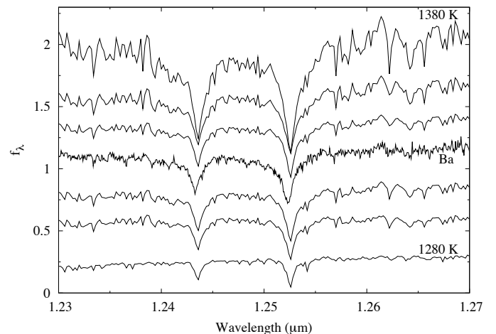
Fig. 17. 1.23\text{--}1.27 \mu\text{m} spectrum of \varepsilon Indi Ba (thicker line, fourth from top) and the [M/H]=-0.2 , \log g=5.50 BT-Settl spectra with T_{\text{eff}}=1280\text{--}1380 K (increasing bottom to top in steps of 20 K). All spectra have been normalised and offset for clarity. Model spectra have been smoothed to 2.4 \text{ \AA} FWHM.
