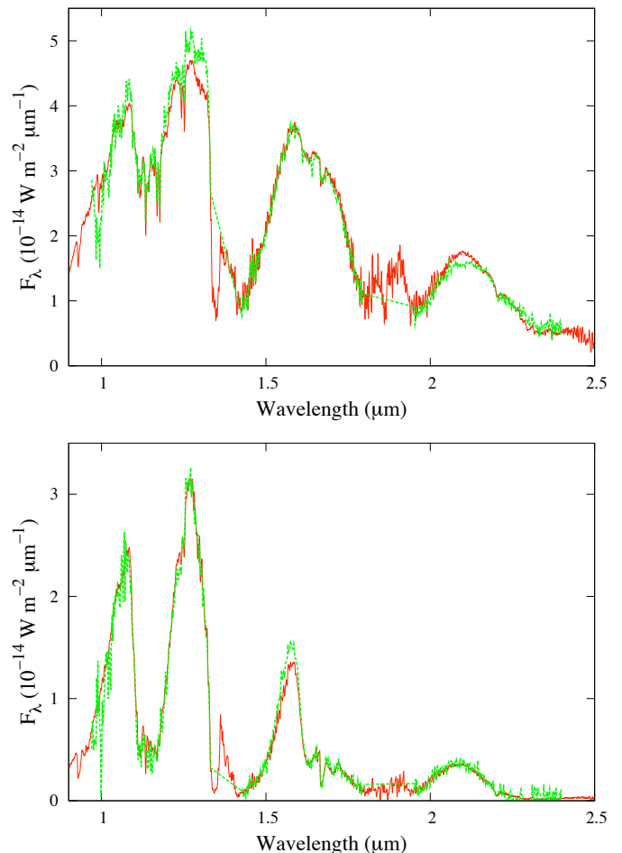
Fig. 2. Our spectra of \varepsilon Indi Ba and Bb (red lines), smoothed to a resolution of 17 \text{ \AA} FWHM and median filtered in the regions of high telluric absorption, compared to the lower resolution spectroscopy of Kasper et al. (2009) (green lines). It is seen that the overall match of the absolute scale is reasonable. Here we have absolutely flux-calibrated using our ISAAC photometric observations, while Kasper et al. (2009) use the 2MASS point source catalogue magnitudes.
