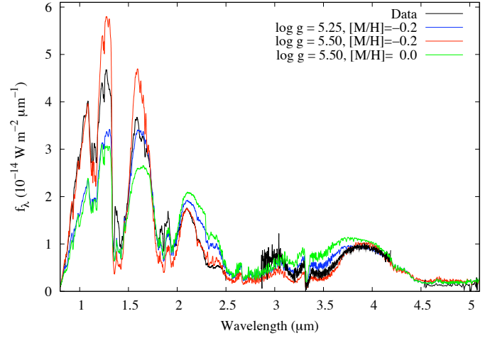
Fig. 20. Near- to thermal-IR spectra of \epsilon Indi Ba (black line), the BT-Settl spectrum ( T_{\text{eff}}=1320 K, \log g=5.50 , [M/H]=-0.2 , red line), the same with \log g=5.25 (blue line), and with \log g=5.50 but with solar metallicity ( [M/H]=0.0 , green line). All spectra have been smoothed to 60 \text{ \AA} FWHM and the observed spectrum median filtered to remove the lowest signal-to-noise points.
