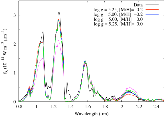
Fig. 21. Near-IR spectra of \epsilon Indi Bb (black line), the BT-Settl spectrum ( T_{\text{eff}}=920\text{K} , \log g=5.25 , [M/H]=-0.2 , red line), the same with \log g=5.00 (blue line), with \log g=5.00 , [M/H]=0.0 (magenta line), and \log g=5.25 , [M/H]=0.0 and (green line). All spectra have been smoothed to 60\text{\AA} FWHM and the observed spectrum median filtered to remove the lowest signal-to-noise points. The thermal-IR spectra have not been shown as there is little to distinguish between models.
