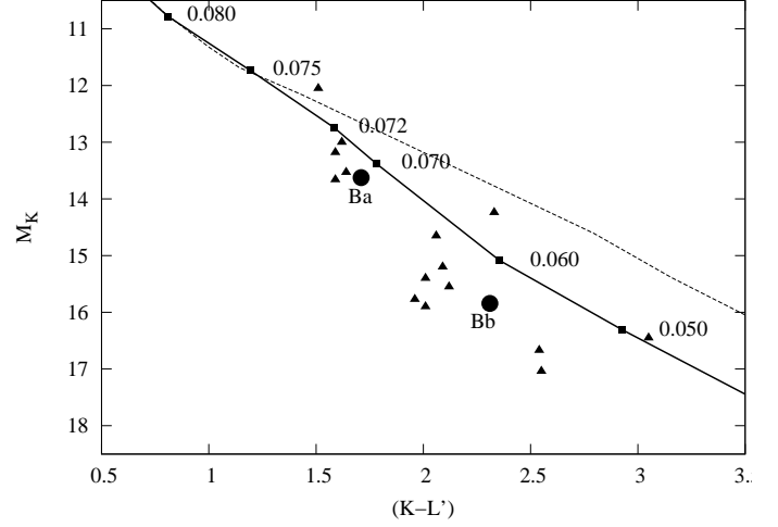
Fig. 13. M_K -( K-L' ) colour-magnitude diagram with the 5 Gyr COND03 isochrone with masses (in M_\odot ) indicated as filled squares. The DUSTY00 5 Gyr isochrone is also shown (upper, dashed line). Symbols are the same as in Fig. 12 with the unlabelled data from Knapp et al. (2004), Chiu et al. (2006), and Golimowski et al. (2004). The data are in the MKO system, whereas the model L' magnitude is in the Johnson-Glass system.
