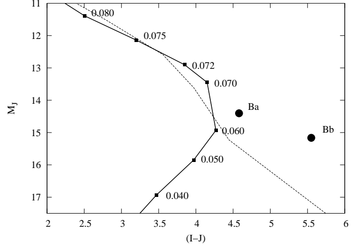
Fig. 14. M_J -( I-J ) colour-magnitude diagram with the 5 Gyr COND03 isochrone with masses (in M_\odot ) indicated as filled squares. The DUSTY00 5 Gyr isochrone is also shown (dashed line). Symbols are the same as in Fig. 12. J -magnitudes are in the MKO system and I -magnitudes use the FORS2 Bessell I filter.
