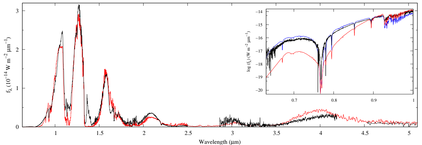
Fig. 23. Optical to thermal-IR spectrum of \varepsilon Indi Bb (black line) and the best-fit BT-Settl spectrum (red line, T_{\text{eff}}=920\text{K} , \log g=5.25 , [M/H]=-0.2 ). The spectra have been smoothed as in Fig. 22. For this late T-dwarf, the depleted alkali model provides the better match to the observed flux levels and spectral morphology in the optical which may be an indication of the formation of feldspars in late-T dwarfs which is not evident in earlier types. No lithium depletion has been implemented in these models.
